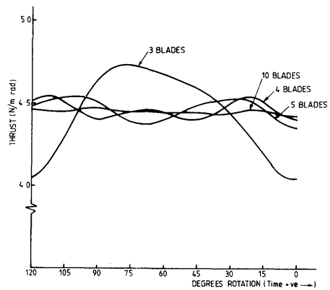
11 c Comparison of Vertical Force on Propeller at Const. Solidity
