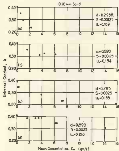
FIG. 3. VARIATION OF THE VON KÁRMÁN UNIVERSAL CONSTANT k WITH CONCENTRATION OF SAND IN THE FLOW IN A FLUME 33 IN. WIDE.
