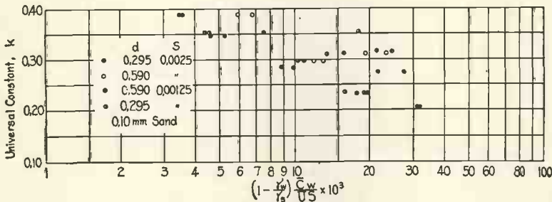
FIG. 6. THE VON KÁRMÁN CONSTANT k PLOTTED AGAINST THE RATIO OF POWER TO SUSPEND SEDIMENT AND POWER TO OVERCOME CHANNEL FRICTION.
