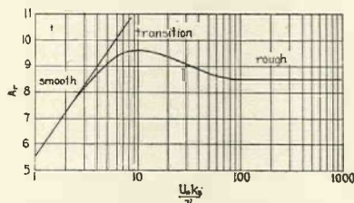
FIG. 5. THE COEFFICIENT A_r FOR ROUGH SURFACES AS A FUNCTION OF THE ROUGHNESS CHARACTERISTIC.
