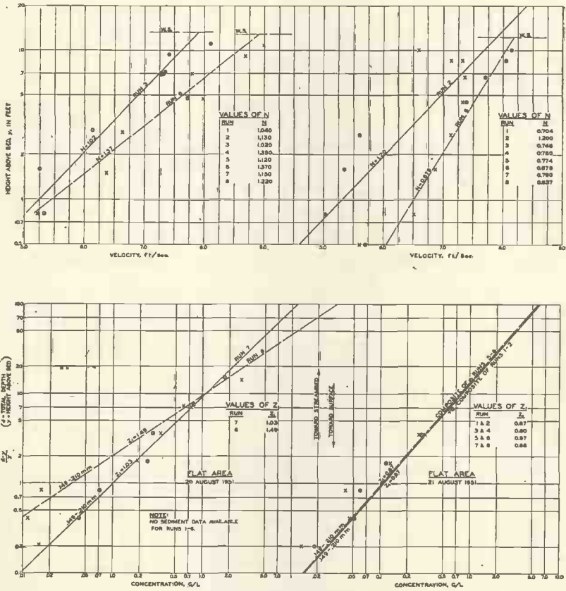
FIG. 11. VARIATION OF VELOCITY AND SEDIMENT DISTRIBUTION WITH VELOCITY CHANGES, MISSOURI RIVER AT OMAHA, NEBRASKA.
