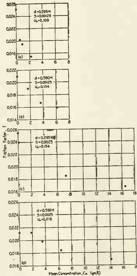
FIG. 1. FRICTION FACTOR OF A FLUME 33 IN. WIDE AS A FUNCTION OF CONCENTRATION OF 0.10 MM SAND IN THE FLOW.
