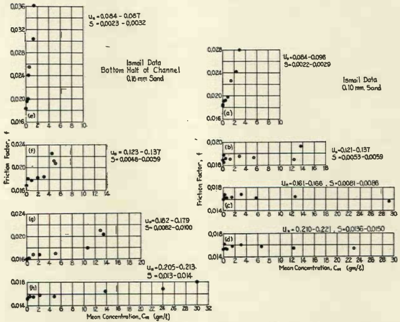
FIG. 2. FRICTION FACTOR OF A RECTANGULAR PIPE 3 IN. X 10-1/2 IN. AS A FUNCTION OF CONCENTRATION OF SAND IN THE FLOW.
