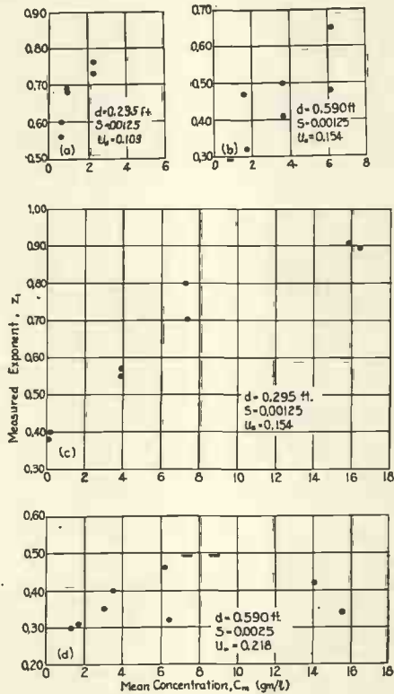
FIG. 8. VARIATION OF THE EXPONENT z_1 WITH CONCENTRATION OF SEDIMENT BEING TRANSPORTED IN A FLUME 33 IN. WIDE.
