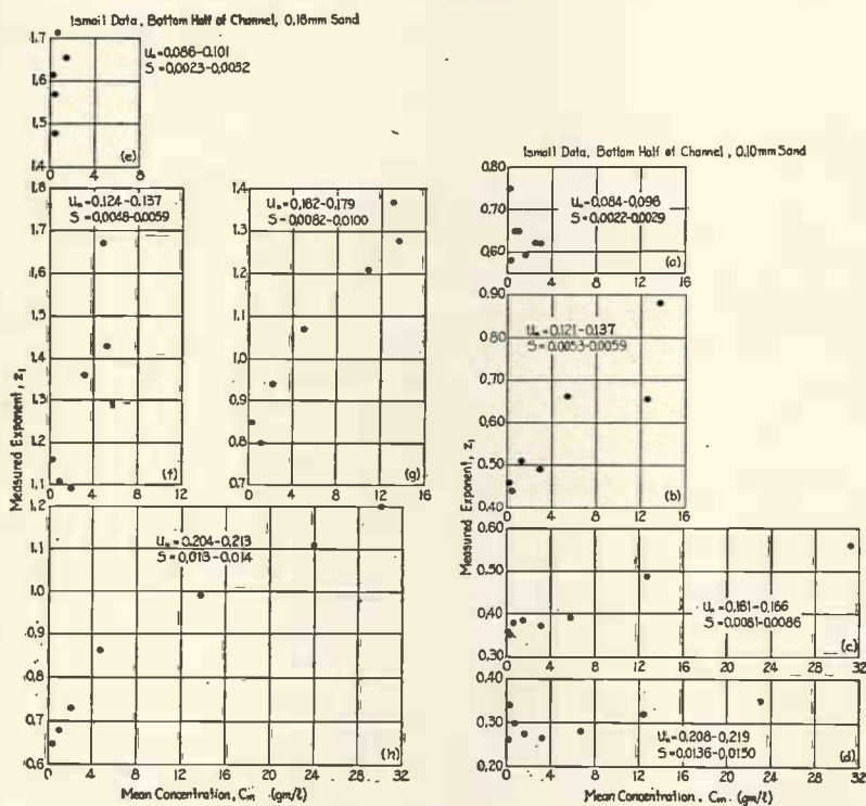
FIG. 9. VARIATION OF THE EXPONENT z_1 WITH CONCENTRATION OF SEDIMENT BEING TRANSPORTED IN A RECTANGULAR PIPE 3 IN. X 10^{-1/2} IN.
