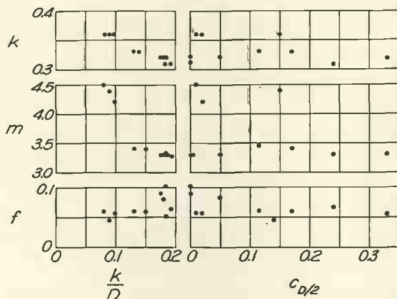
FIG. 13. RELATION OF CONCENTRATION WITH RELATIVE ROUGHNESS, FLUME MEASUREMENTS AT THE IOWA INSTITUTE OF HYDRAULIC RESEARCH.
