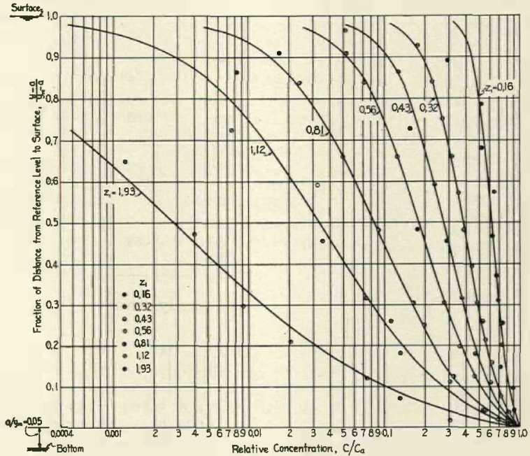
FIG. 7. VERTICAL DISTRIBUTION OF RELATIVE CONCENTRATION OF SEDIMENT OVER A WIDE RANGE OF CONDITIONS OF FLOW AND SEDIMENT SIZE.
