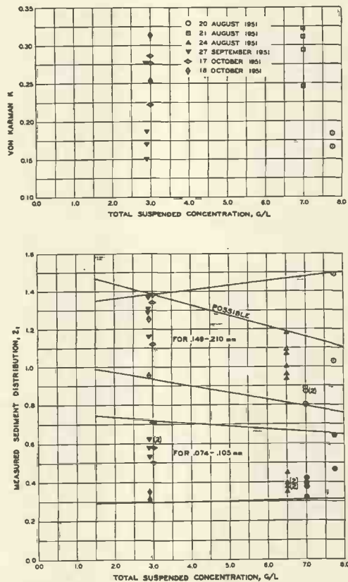
FIG. 10. VARIATION IN k AND z_1 WITH CONCENTRATION, MISSOURI RIVER AT OMAHA, NEBRASKA.
