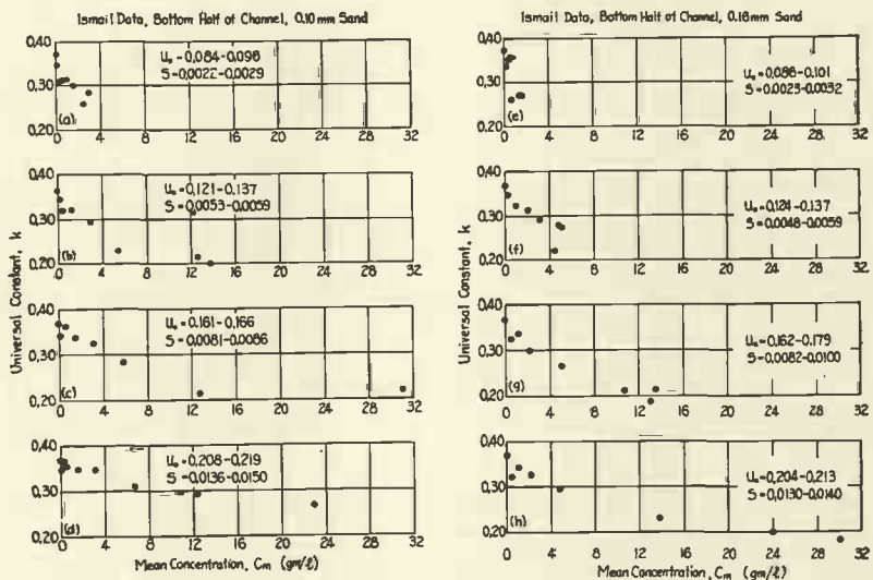
FIG. 4. VARIATION OF THE VON KÁRMÁN UNIVERSAL CONSTANT k WITH CONCENTRATION OF SAND IN THE FLOW IN A RECTANGULAR PIPE 3 IN. X 10\frac{1}{2} IN.
