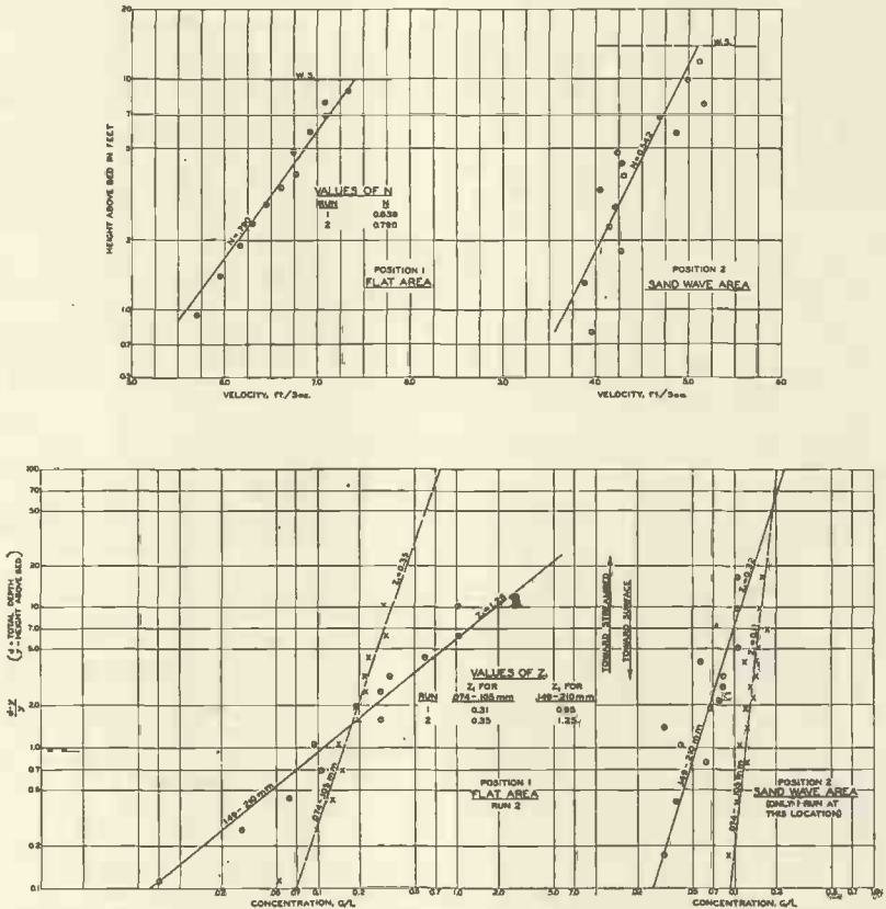
FIG. 12. VARIATION OF VELOCITY AND SEDIMENT DISTRIBUTION WITH BED FORM, MISSOURI RIVER AT OMAHA, NEBRASKA.
